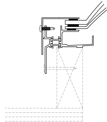
Sill Section
